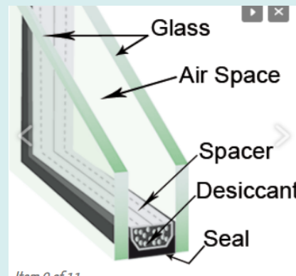
Insulated Glass Diagram
