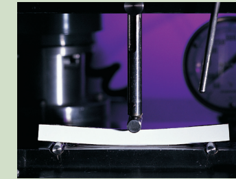
AAMA Temperature Deflection Test
